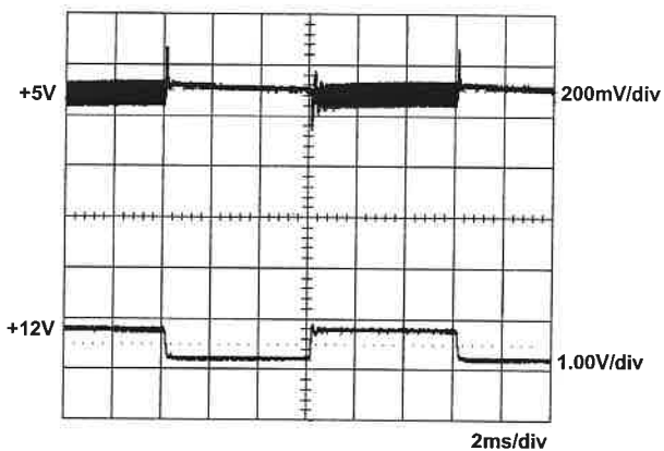
+5V step from 2A to 10A other output at 60% load
