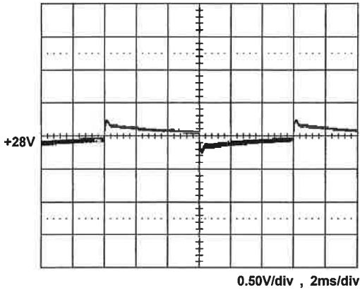
+28V step from 0.76A to 3.8A
